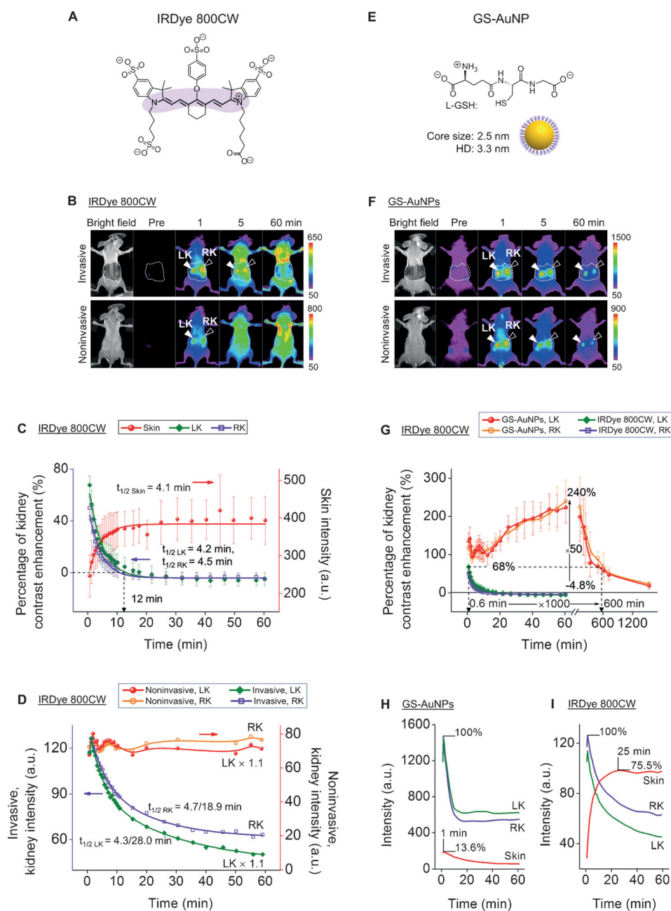
Figure 2. Comparison of renal-clearable NIR-emitting IRDye 800CW and GS-AuNPs in noninvasive kidney imaging. A) Chemical structure of IRDye 800CW. B) Whole-body invasive and noninvasive fluorescence images of mice before and after iv injection of IRDye 800CW (Ex/Em filters: 710/790 nm). The skin-removed areas were marked by dashed white line. LK, left kidney; RK, right kidney. C) Time-course changes in skin intensity and percentage of kidney-contrast enhancements of mice after iv injection of IRDye 800CW. N=3 , mean \pm s.d. D) Time-fluorescence intensity curves (TFICs) of kidneys obtained from noninvasive and invasive fluorescence imaging of mice after iv injection of IRDye 800CW. E) Representation of GS-AuNPs. F) Whole-body invasive and noninvasive fluorescence images of mice before and after iv injection of GS-AuNPs (Ex/Em filters: 710/830 nm). G) Comparison of time-dependent kidney contrast enhancements in percentage after GS-AuNPs and IRDye 800CW injection, respectively. N=3 , mean \pm s.d. H, I) TFICs of kidneys and skin obtained from invasive imaging after iv injection of GS-AuNPs (H) and IRDye 800CW (I).
